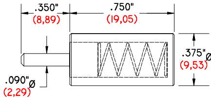
GI-093/090 DTPA RED DELTRIN TOOLING PIN ASSEMBLY
