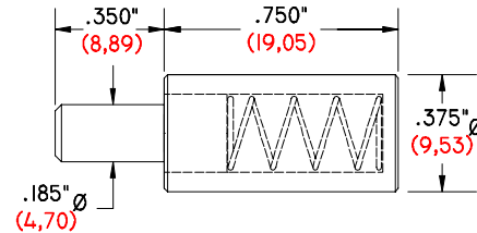
GI-187/185 DTPA GREEN DELTRIN TOOLING PIN ASSEMBLY
