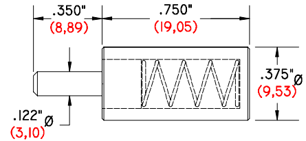
GI-125/122 DTPA PURPLE DELTRIN TOOLING PIN ASSEMBLY
