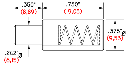
GI-246/242 DTPA BLUE DELTRIN TOOLING PIN ASSEMBLY
