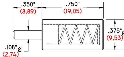
GI-III/108 DTPA PINK DELTRIN TOOLING PIN ASSEMBLY
