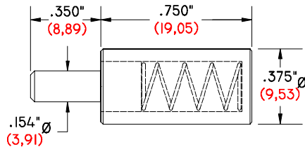
GI-157/154 DTPA YELLOW DELTRIN TOOLING PIN ASSEMBLY
