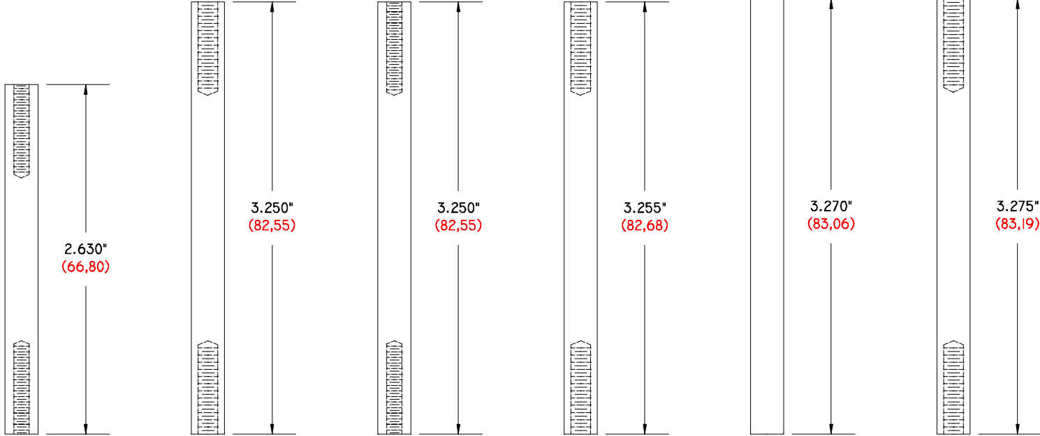
GI-2630-250/6-32 DP 2.630" (66,80) LONG .250" (6,35) Ø O. D. 6-32 THREAD DELRIN POST
