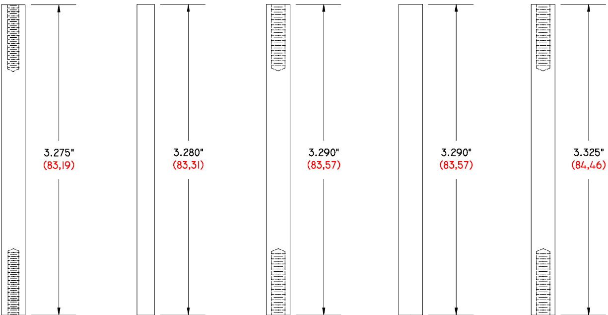
GI-3275-250/6-32 DP 3.275" (83,19) LONG .250" (6,35) Ø O. D. 6-32 THREAD DELRIN POST
