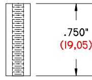
GI-750-250/6-32 DS .750" (19,05) LONG .250" (6,35) Ø O. D. 6-32 THREAD DELRIN SPACER
