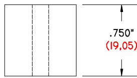
GI-750-750/170 DS .750" (19,05) LONG .750" (19,05) Ø O. D. .170" (4,32) Ø I. D. DELRIN SPACER
