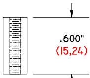
GI-600-250/6-32 DS .600" (15,24) LONG .250" (6,35) Ø O. D. 6-32 THREAD DELRIN SPACER
