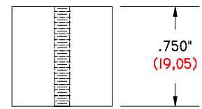
GI-750-750/6-32 DS .750" (19,05) LONG .750" (19,05) Ø O. D. 6-32 THREAD DELRIN SPACER
