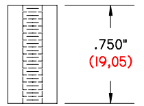
GI-750-375/8-32 DS .750" (19,05) LONG .375" (9,53) Ø O. D. 8-32 THREAD DELRIN SPACER
