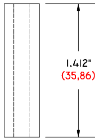
GI-1412-375/170 DS 1.412" (35,86) LONG .375" (9,53) Ø O. D. .170" (4,32) Ø I. D. DELRIN SPACER
