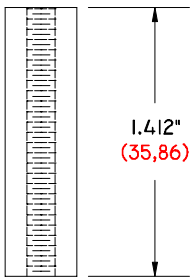
GI-1412-375/8-32 DS 1.412" (35,86) LONG .375" (9,53) Ø O. D. 8-32 THREAD DELRIN SPACER
