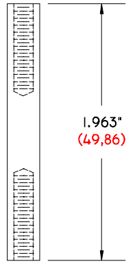
GI-1963-250/8-32 DP 1.963" (49,86) LONG .250" (6,35) Ø O. D. 8-32 THREAD DELRIN POST
