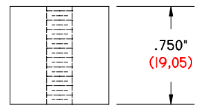
GI-750-750/10-24 DS .750" (19,05) LONG .750" (19,05) Ø O. D. 10-24 THREAD DELRIN SPACER
