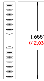
GI-1655-250/8-32 DP 1.655" (42,03) LONG .250" (6,35) Ø O. D. 8-32 THREAD DELRIN POST
