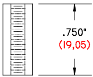
GI-750-312/8-32 DS .750" (19,05) LONG .312" (7,92) Ø O. D. 8-32 THREAD DELRIN SPACER
