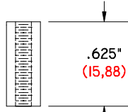
GI-625-250/6-32 DS .625" (15,88) LONG .250" (6,35) Ø O. D. 6-32 THREAD DELRIN SPACER
