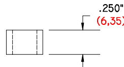
GI-250-375/257 DS .250" (6,35) LONG .375" (9,53) Ø O. D. .257" (6,53) Ø I. D. DELRIN SPACER
