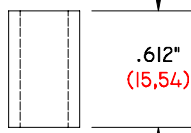
GI-612-375/257 DS .612" (15,54) LONG .375" (9,53) Ø O. D. .257" (6,53) Ø I. D. DELRIN SPACER
