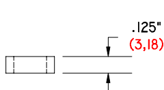
GI-125-375/257 DS .125" (3,18) LONG .375" (9,53) Ø O. D. .257" (6,53) Ø I. D. DELRIN SPACER
