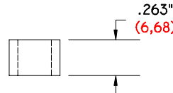
GI-263-375/257 DS .263" (6,68) LONG .375" (9,53) Ø O. D. .257" (6,53) Ø I. D. DELRIN SPACER
