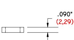
GI-090-375/257 DS .090" (2,29) LONG .375" (9,53) Ø O. D. .257" (6,53) Ø I. D. DELRIN SPACER
