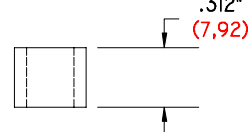
GI-312-375/257 DS .312" (7,92) LONG .375" (9,53) Ø O. D. .257" (6,53) Ø I. D. DELRIN SPACER
