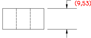
GI-375-750/257 DS .375" (9,53) LONG .750" (19,05) Ø O. D. .257" (6,53) Ø I. D. DELRIN SPACER
