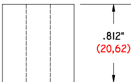
GI-812-750/257 DS .812" (20,62) LONG .750" (19,05) Ø O. D. .257" (6,53) Ø I. D. DELRIN SPACER
