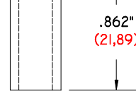
GI-862-375/257 DS .862" (21,89) LONG .375" (9,53) Ø O. D. .257" (6,53) Ø I. D. DELRIN SPACER
