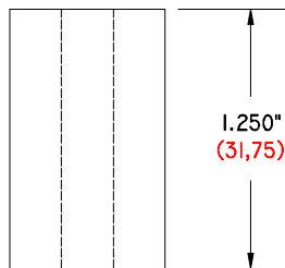
GI-1250-750/257 DS 1.250" (31,75) LONG .750" (19,05) Ø O. D. .257" (6,53) Ø I. D. DELRIN SPACER
