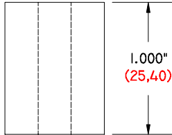
GI-1000-750/257 DS 1.000" (25,40) LONG .750" (19,05) Ø O. D. .257" (6,53) Ø I. D. DELTRIN SPACER
