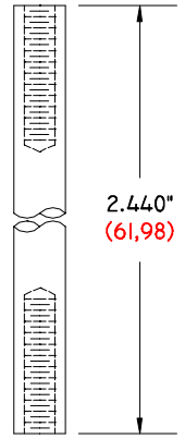
GI-2440-250/8-32 DS 2.440" (61,98) LONG .250" (6,35) Ø O. D. 8-32 THREAD DELTRIN SPACER
