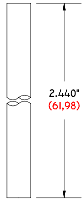
GI-2440-250 FL 2.440" (61,98) LONG .250" (6,35) Ø O. D. DELTRIN POST
