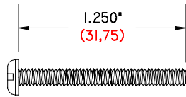
GI-1 1/4-6-32 PHNS 1.250" (31,75) LONG 6-32 THREAD PAN HEAD NYLON SCREW
