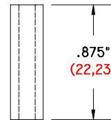
GI-875-250/125 DS .875" (22,23) LONG .250" (6,35) Ø O. D. .125" (3,18) Ø I. D. DELRIN SPACER
