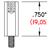
GI-750-250/6-32 MFHS .750" (19,05) LONG .250" (6,35) HEXAGON 6-32 THREAD MALE - FEMALE HEXAGON SPACER
