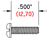
GI-1/2-6-32 PHNS .500" (12,70) LONG 6-32 THREAD PAN HEAD NYLON SCREW
