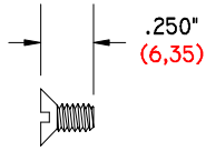
GI-1/4-6-32 FHNS .250" (6,35) LONG 6-32 THREAD FLAT HEAD NYLON SCREW
