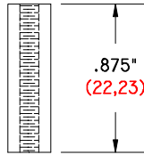
GI-875-250/6-32 DS .875" (22,23) LONG .250" (6,35) Ø O. D. 6-32 THREAD DELRIN SPACER
