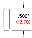
GI-1/2-1/8 DP .500" (12,70) LONG .125" (3,18) Ø O. D. DOWEL PIN
