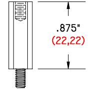
GI-875-250/6-32 MFHS .875" (22,23) LONG .250" (6,35) HEXAGON 6-32 THREAD MALE - FEMALE HEXAGON SPACER
