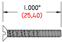
GI-1-6-32 FHSS 1.000" (25,40) LONG 6-32 THREAD FLAT HEAD STAINLESS STEEL SCREW
